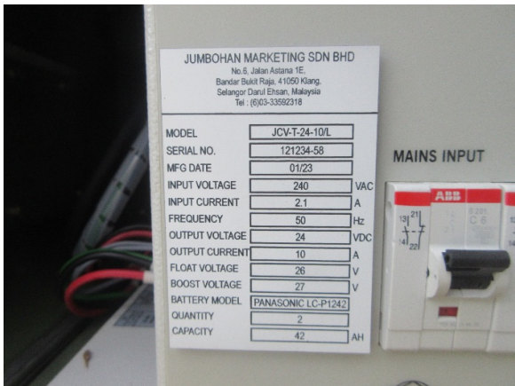
BATTERY CHARGER NAMEPLATE
